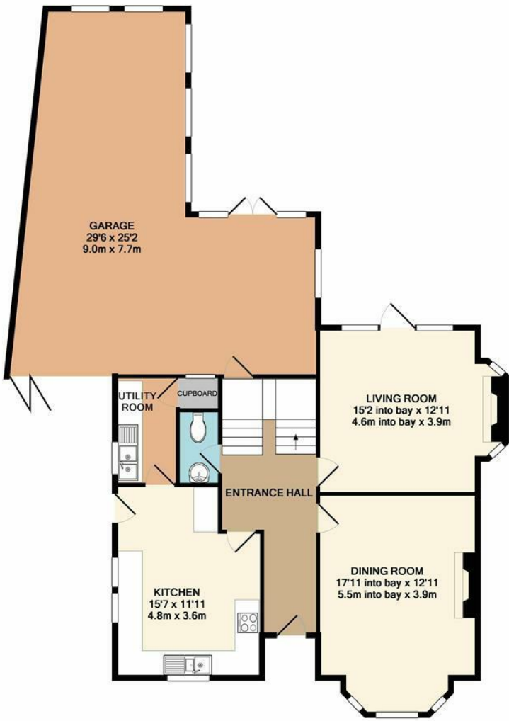
GROUND FLOOR APPROX. FLOOR AREA 1321 SQ.FT. (122.7 SQ.M.)
